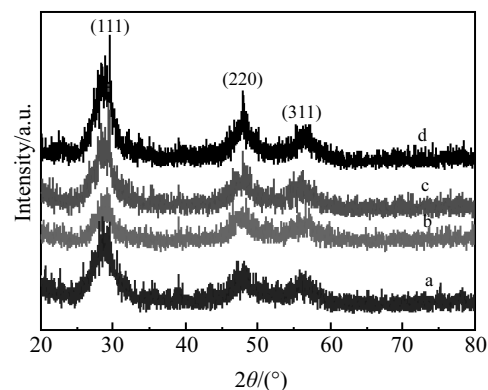
Fig.1 XRD patterns of \text{ZnS:Er/Yb} nanoparticles: (a) \text{ZnS:Er} (1 mol%), \text{Yb} (1 mol%), (b) \text{ZnS:Er} (1 mol%), \text{Yb} (2 mol%), (c) \text{ZnS:Er} (1 mol%), \text{Yb} (3 mol%), and (d) \text{ZnS:Er} (1 mol%), \text{Yb} (4 mol%)
