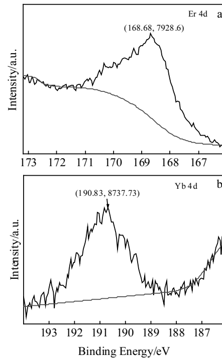
Fig.4 XPS detail scans of Er 4d (a) and Yb 4d (d) of ZnS nanocrystals
