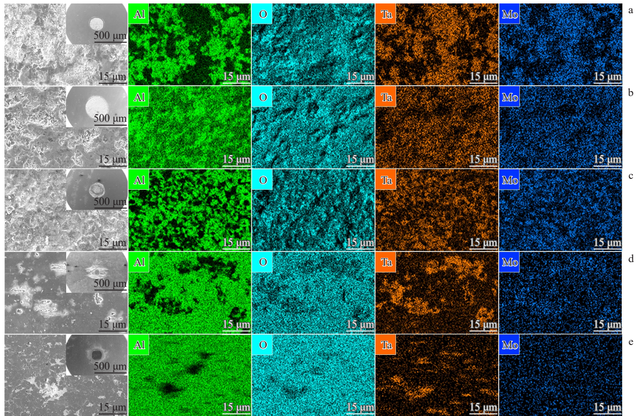
Fig.10 Worn surface morphologies and corresponding EDS element mappings of \text{Al}_2\text{O}_3 balls corresponding to BN5 composite at different temperatures: (a) RT, (b) 300 °C, (c) 600 °C, (d) 800 °C, and (e) 1000 °C
