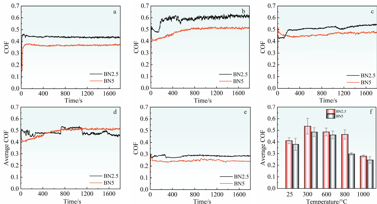
Fig.5 COF curves (a–e) and average COF values (f) of BN2.5 and BN5 ceramic-reinforced RHEA composites at different temperatures: (a) RT, (b) 300 °C, (c) 600 °C, (d) 800 °C, and (e) 1000 °C
