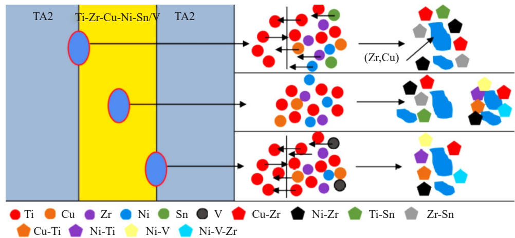
图7 Ti-Zr-Cu-Ni-Sn/V 钎料钎焊 TA2 钛合金界面冶金反应示意图 Fig.7 Schematic diagram of metallurgical reaction at the brazing interface of TA2 titanium alloy with Ti-Zr-Cu-Ni-Sn/V filler metals
