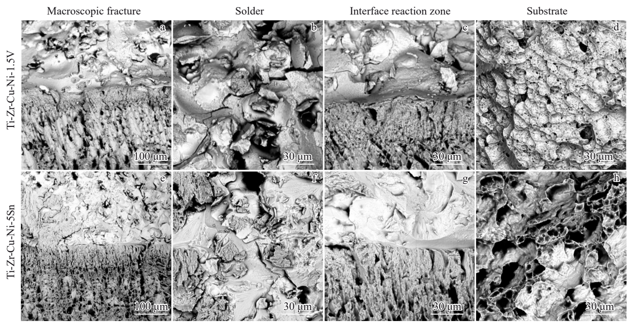
图6 TA2 钛合金钎接头拉伸断口形貌 Fig.6 Tensile fracture morphologies of TA2 titanium alloy brazed joints
