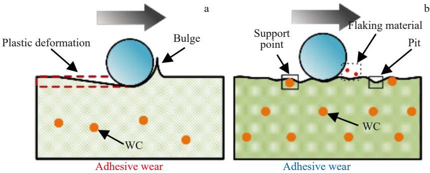
图11 涂层磨损行为演变示意图 Fig.11 Schematic diagram of the evolution of coating wear behavior: (a) low WC content and (b) high WC content
