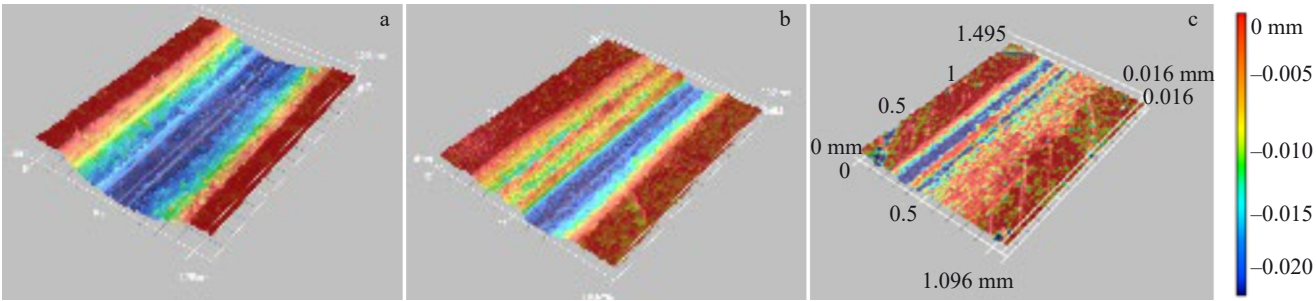
图12 磨损表面的3D轮廓图像 Fig.12 3D contour images of the worn surface: (a) WC 10 , (b) WC 20 , and (c) WC 40
