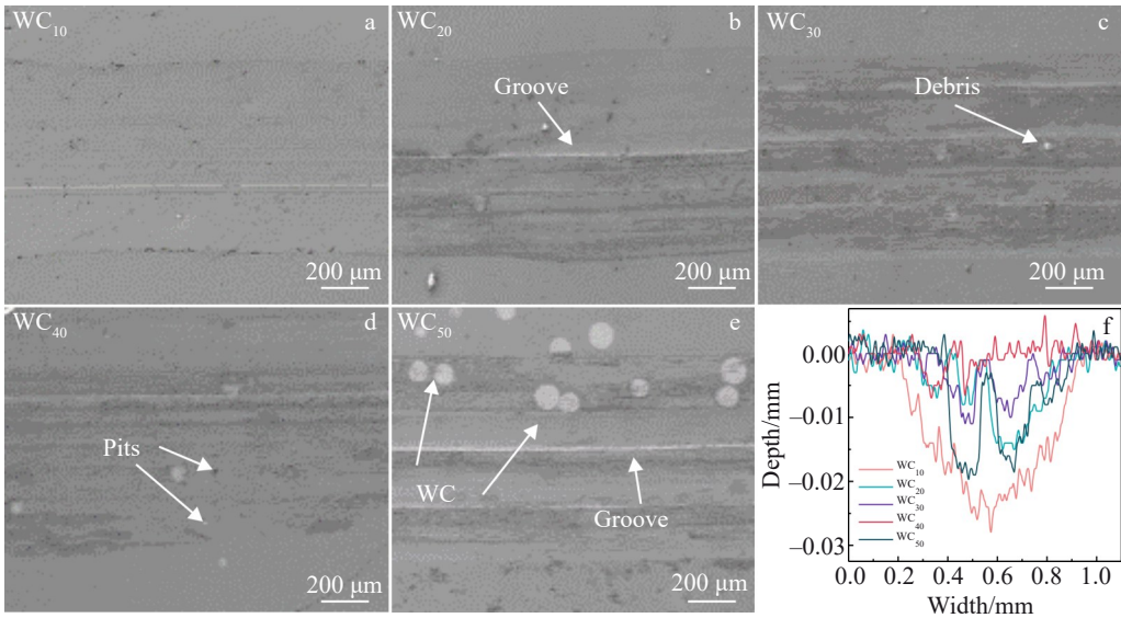
图10 磨损表面的SEM图像与磨痕的深度分布 Fig.10 SEM images of the worn surface (a–e) and depth distribution of the worn surface (f)
