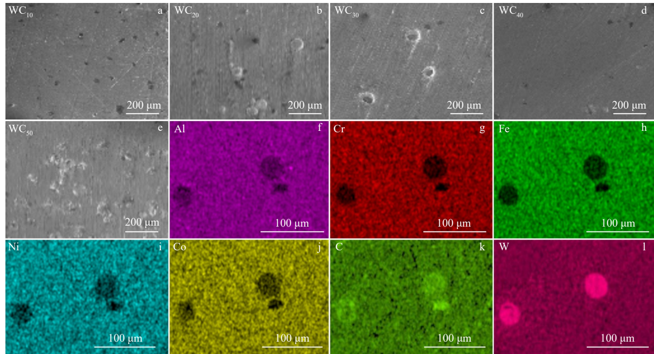
图2 不同WC含量涂层的SEM照片和WC 40 涂层EDS面扫描结果 Fig.2 SEM images of the coatings with different WC contents (a-e) and element mappings of WC 40 coating (f-l)
