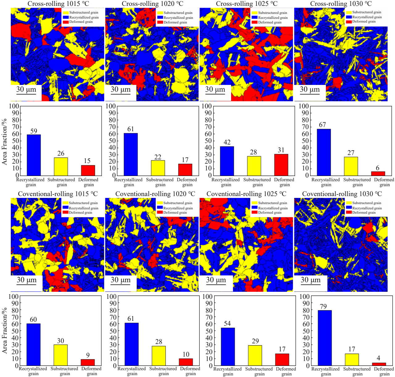
图12 固溶温度对成品板材再结晶晶粒分数的影响 Fig.12 Effect of solution temperature on the fraction of recrystallized grains in finished plate
