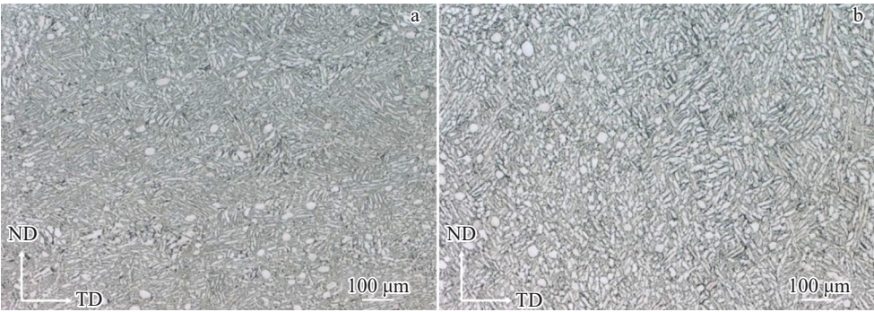
图1 初始板坯组织金相照片 Fig.1 Metallographic photograph of the initial slab structure: (a) surface and (b) core
