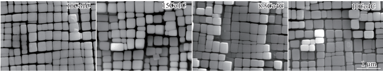
图8 4种合金热处理态的 \gamma' 相形貌 Fig.8 Morphologies of the \gamma' phase in four heat-treated alloys
