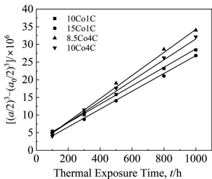
图 10 4 种合金在 1000 °C 长期时效过程中 \gamma' 相的粗化速率 Fig.10 Coarsening rate of \gamma' phase in four alloys during long-term aging at 1000 °C
