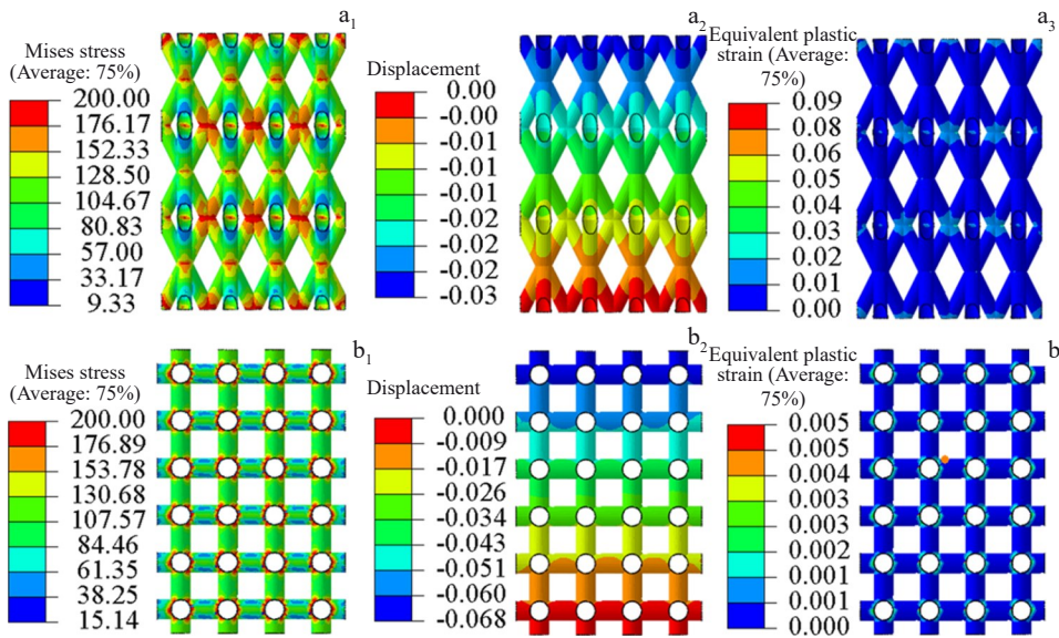
图 11 点阵结构的应力、位移及等效塑性应变分布图 Fig.11 Distributions of Mises stress (a 1 –b 1 ), displacement (a 2 –b 2 ), and equivalent plastic strain (a 3 –b 3 ) of the lattice structure: (a 1 –a 3 ) tetrahedral lattice structure and (b 1 –b 3 ) simple cubic lattice structure
