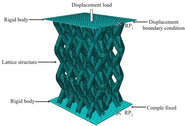
图 10 四面体型点阵结构有限元模型 Fig.10 Finite element model of tetrahedral lattice structure
